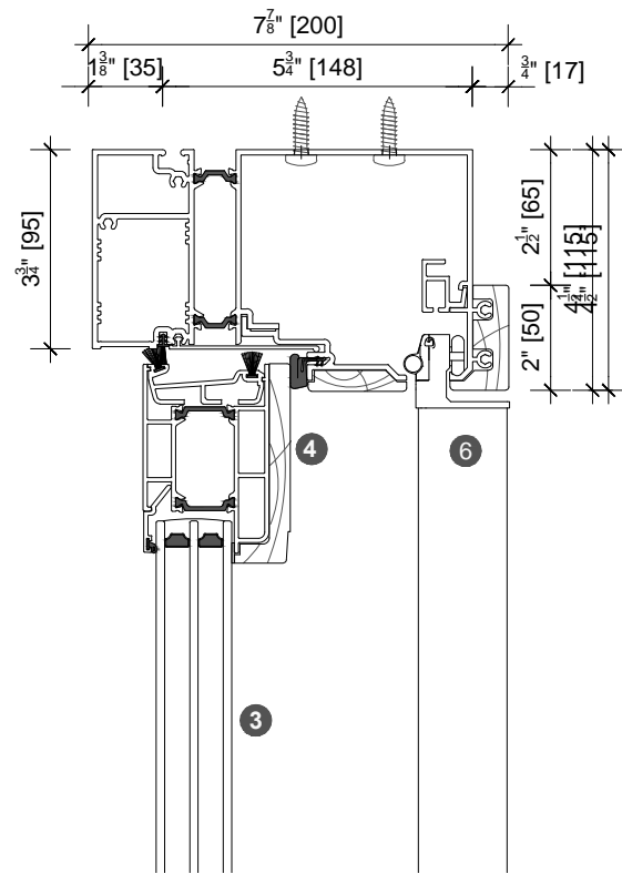
3. head detail
