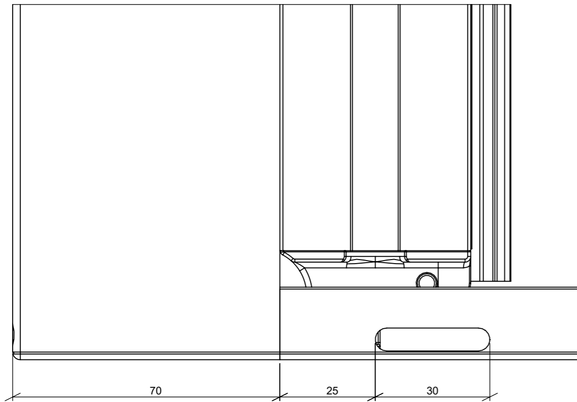
Screened Jamb
