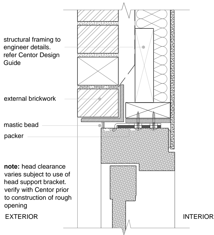
2. head detail
