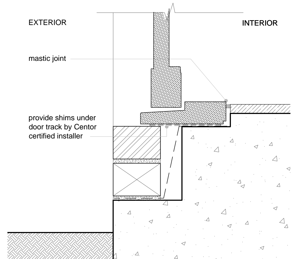
4. sill detail
