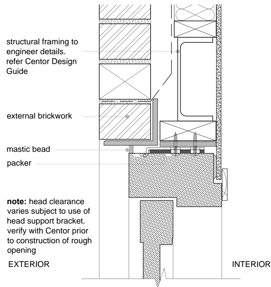
3. head detail
