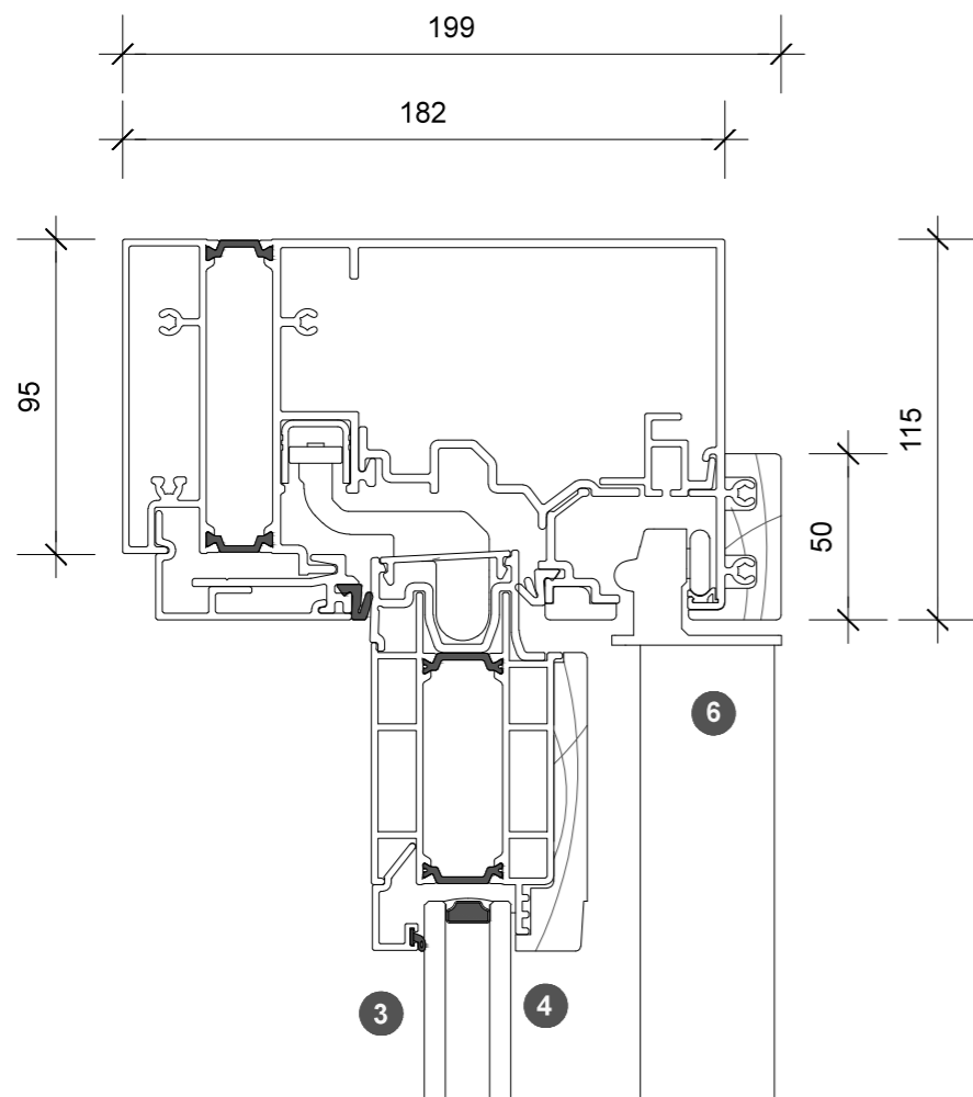
4. head detail
