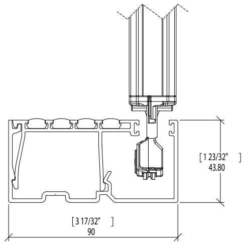
S1 Head and Sill Details
