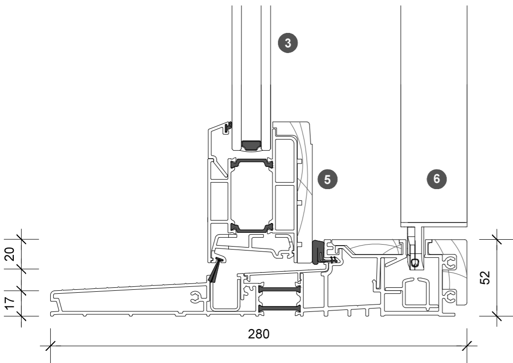
3. head detail
