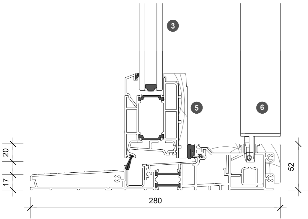
3. head detail
