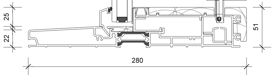
5. sill detail
