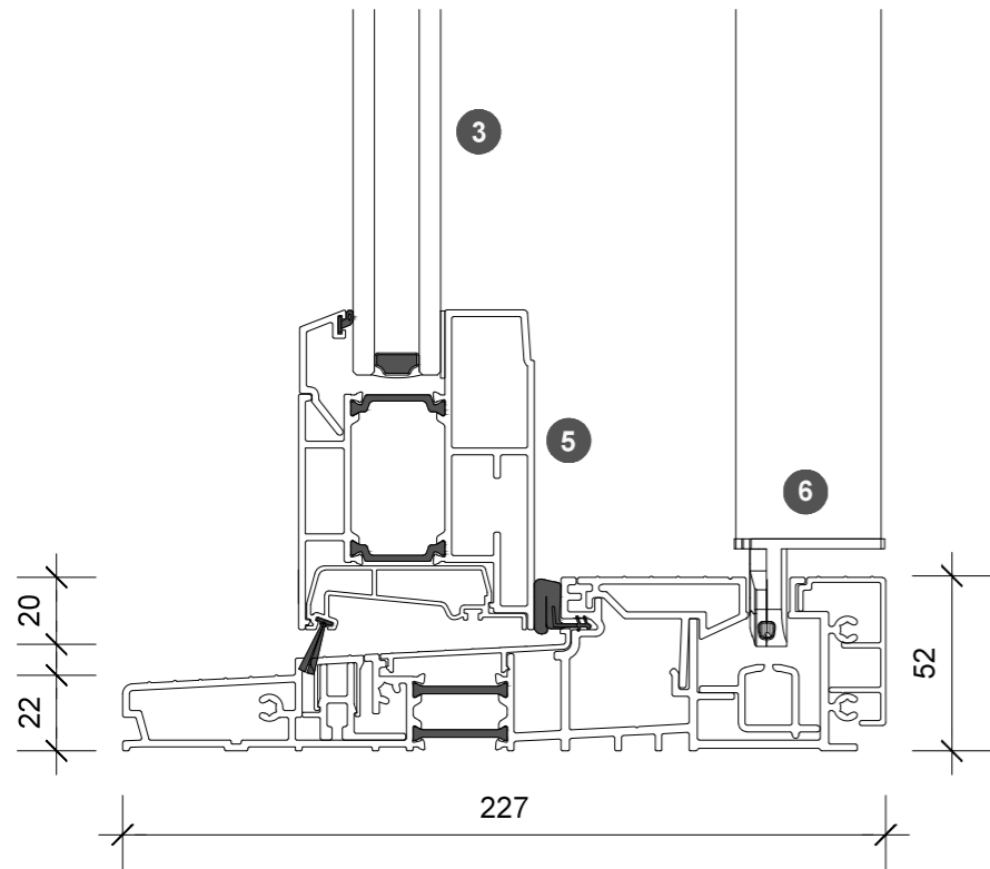
3. head detail
