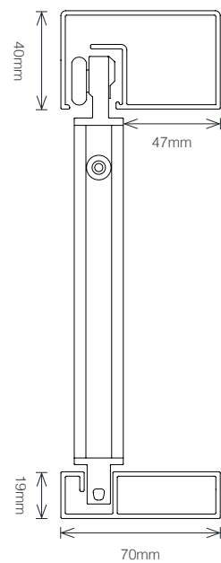
Cross section
