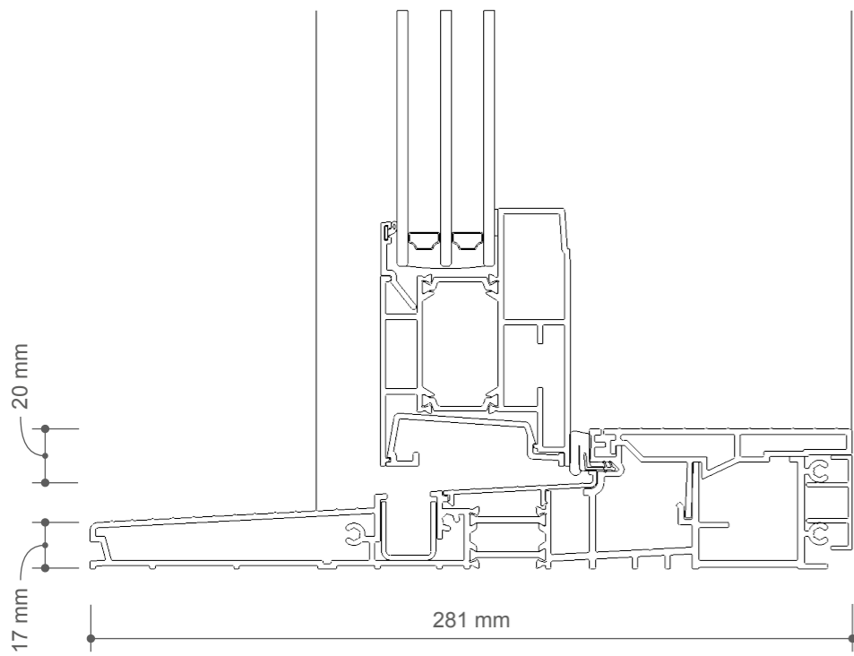
4. Sill detail
