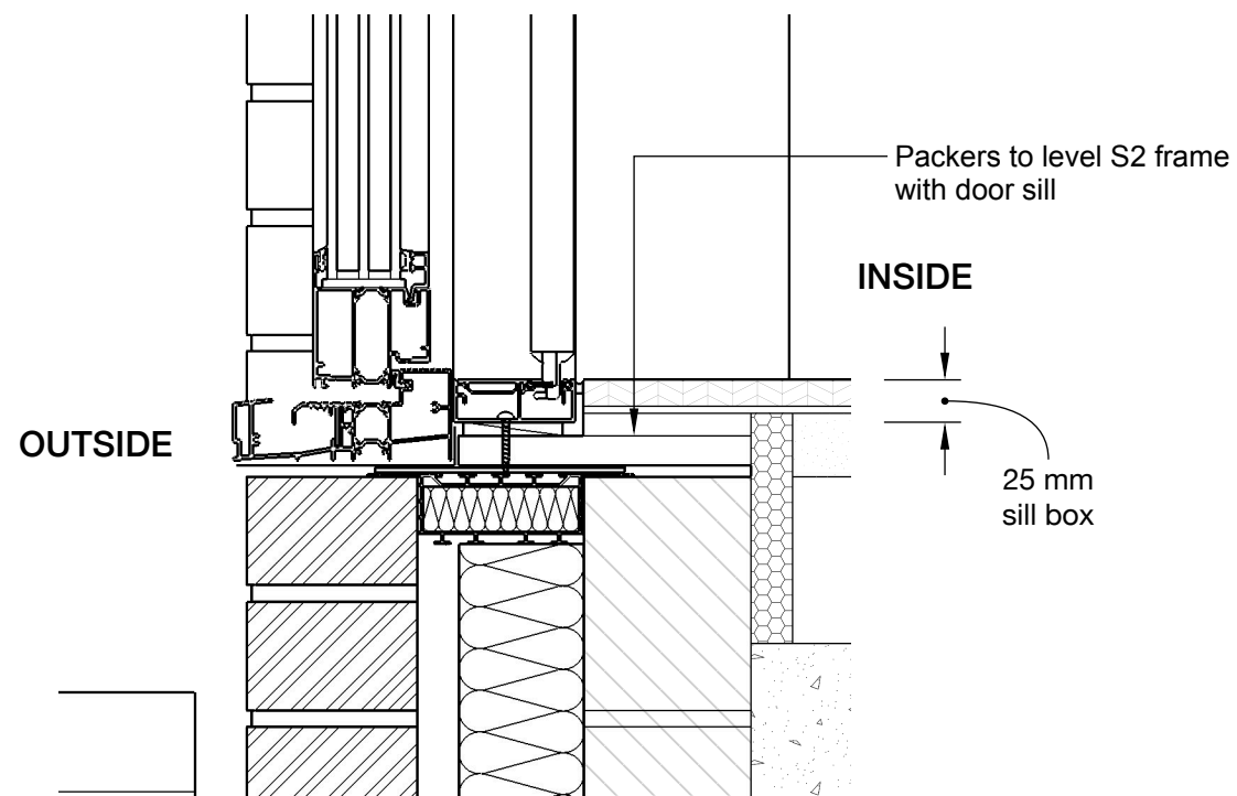
Vertical section Sill
