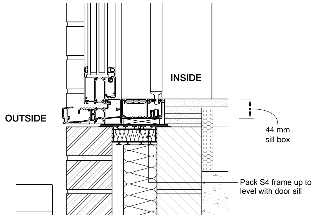
Vertical section Sill
