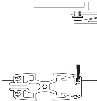
Side Brush Seal (SEL-042)
