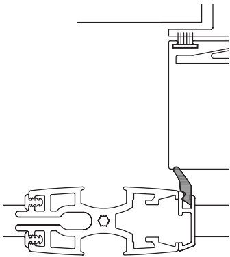
Side Q-Lon Seal (QL7066)
