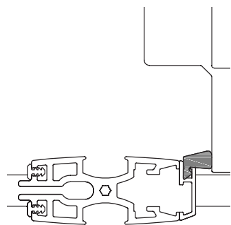
Off-Center Front Seal (AQ109)
