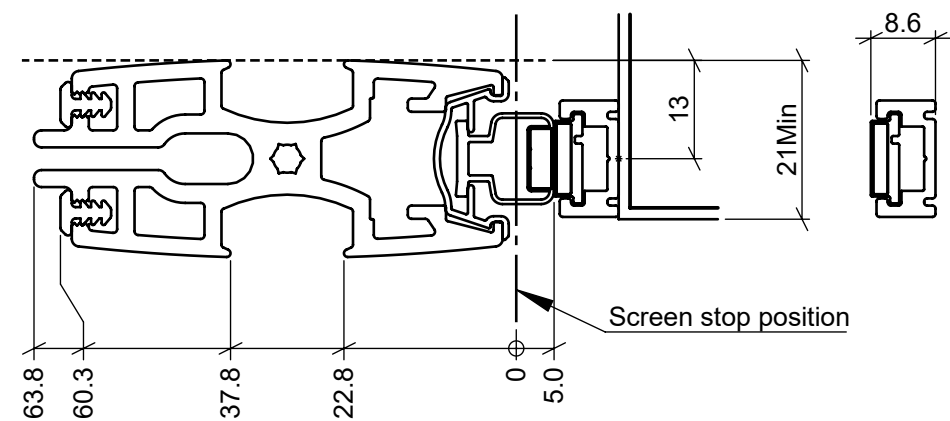
Straight magnet with 8mm adaptor
