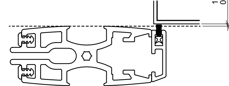
8mm Brush seal SEL-043
