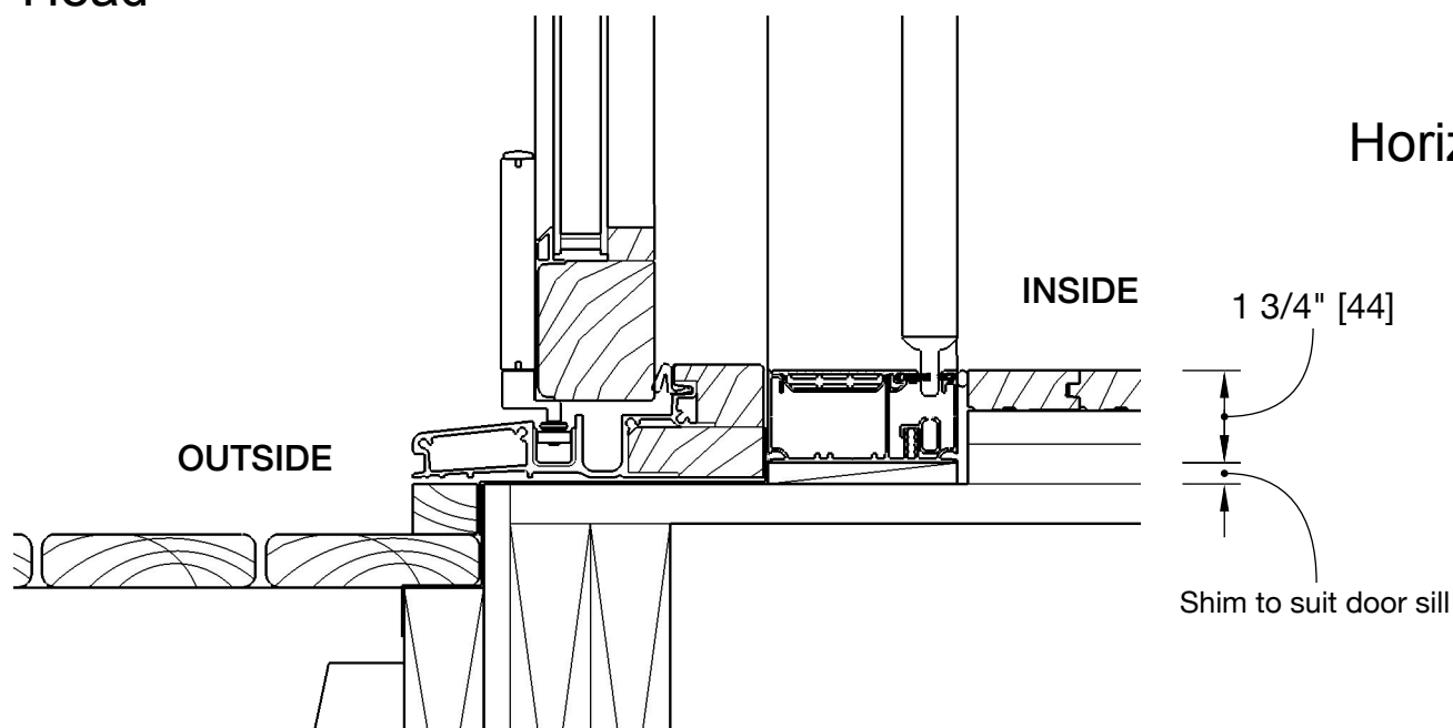
Vertical section Sill
