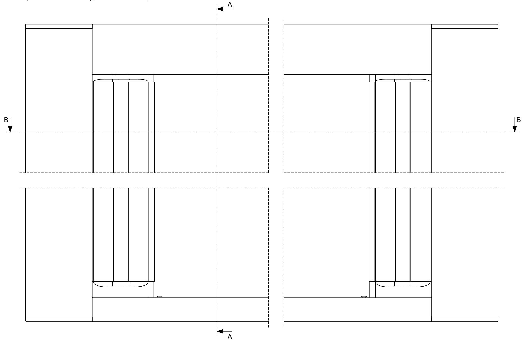
SECTION B-B
