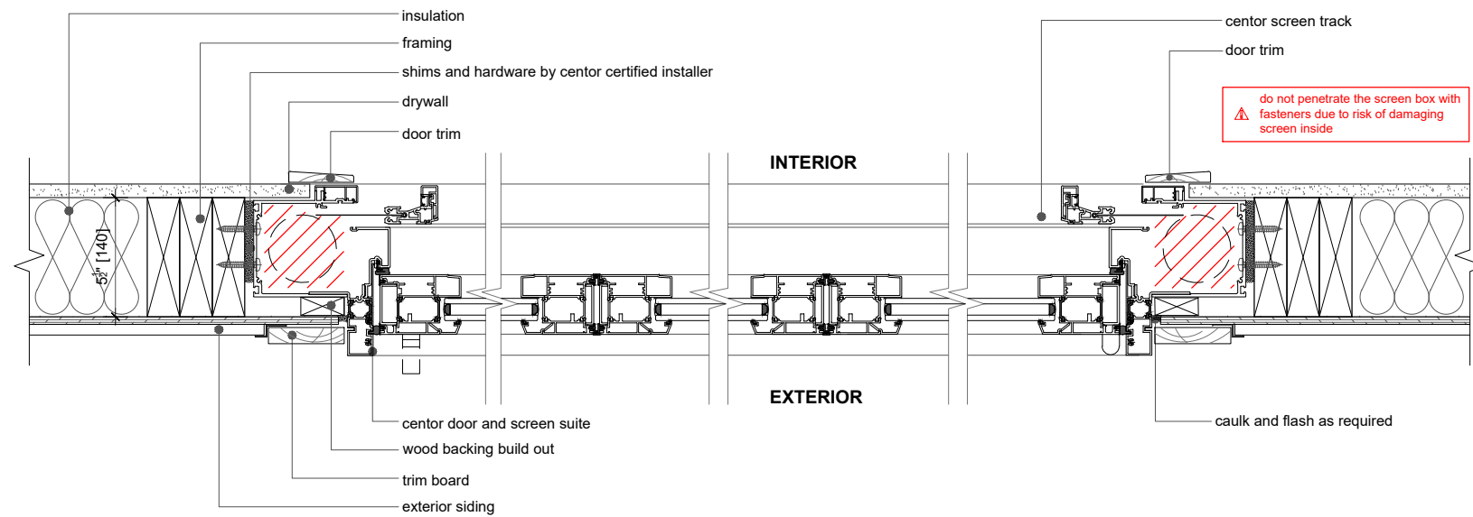
1 jamb detail plan 1 1/2" = 1'-0"
