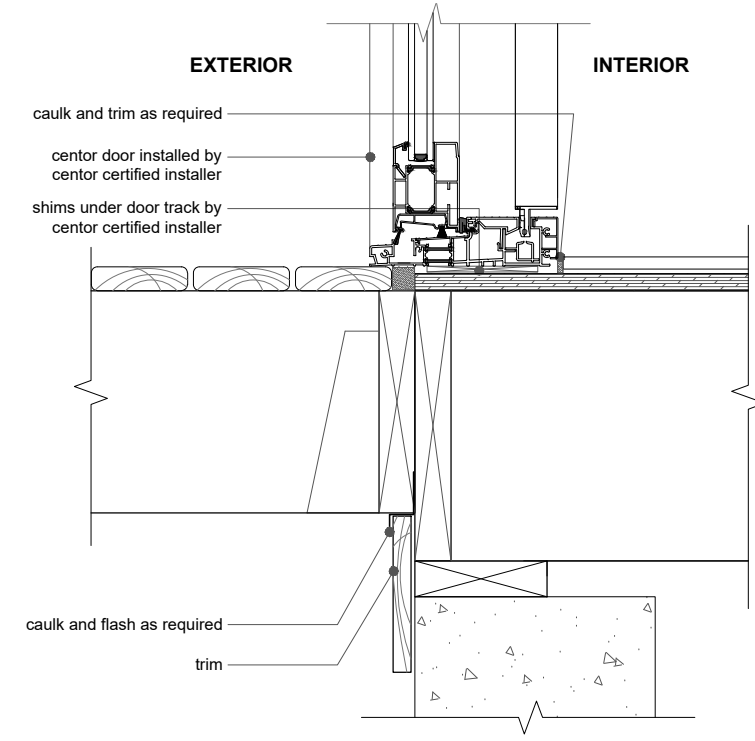
3 sill detail
