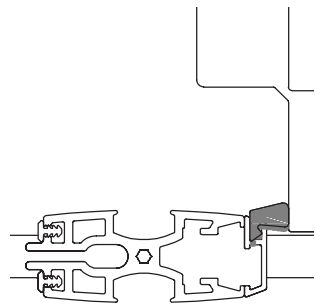
Off-Center Front Seal (AQ109)
