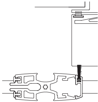
Side Brush Seal (SEL-042)
