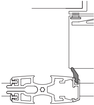
Side Q-Lon Seal (QL7066)
